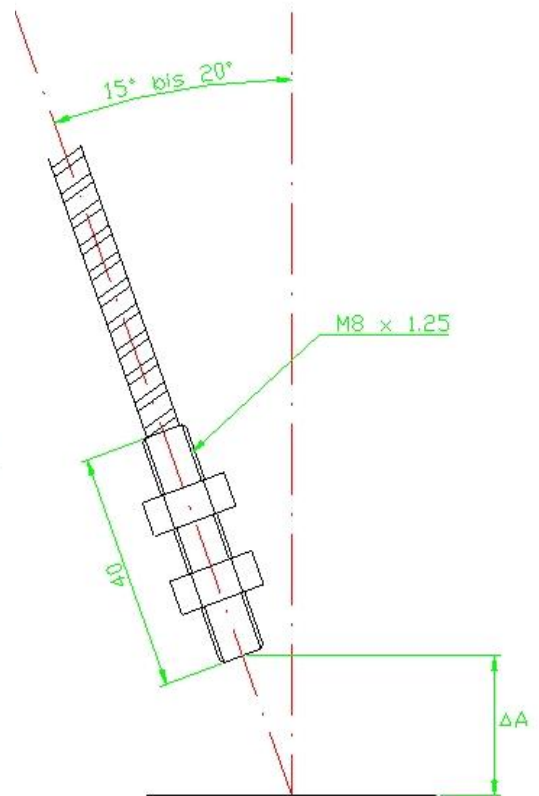
Mounting of light guide
